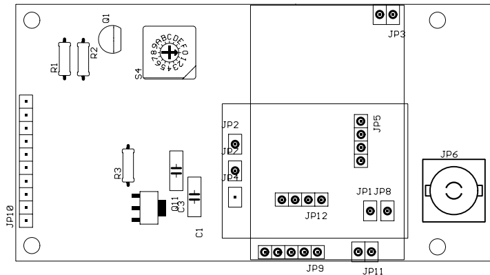
Figure 6: TLC2, RLC2 and HVR2 Module Carrier Board
