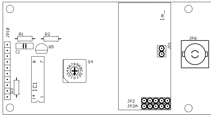
Figure 5: LMT2 or LMR2 Module Carrier Board
