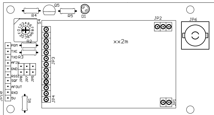
Figure 3: TX1M/RX1M, TX2M/RX2M or TR2M Module Carrier Board
