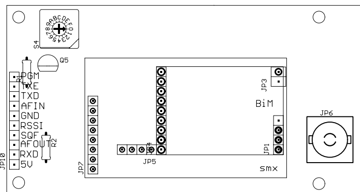
Figure 4: BiM1, NiM2, SMX1 or SMX2 Module Carrier Board
